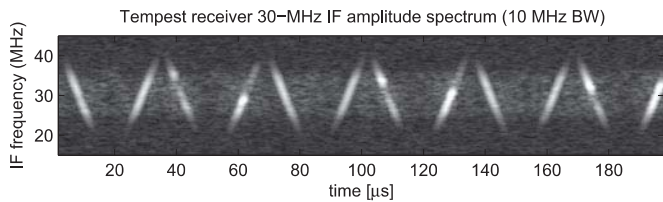
Fig. 5. IF spectrum of 15LCD25 emission (30 MHz IF \pm 690 MHz RF, 10 MHz bandwidth) showing triangle-wave frequency modulation of pixel clock.
