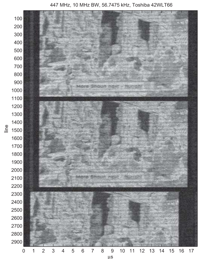
Fig. 7. Toshiba 42WLT66 emissions while receiving BBC1 (PAL).
