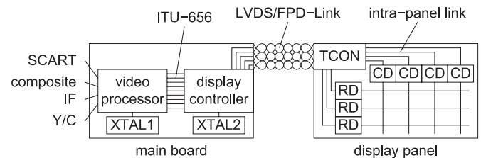
Fig. 2. Typical structure of an LCD TV set.
